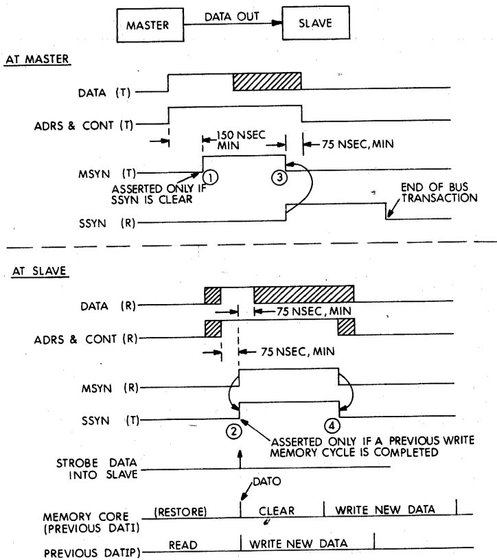
Figure 5-9 DATO & DATOB Timing Diagram
