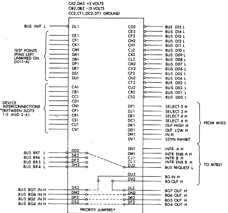
Device Control as Wired in the DD11-A
