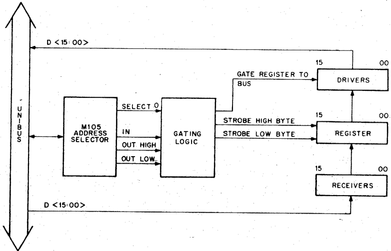
Figure 7-1 Basic Interface (block diagram)
