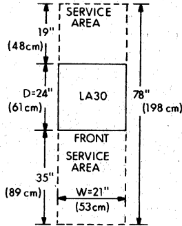
Figure 8-3 Space for LA30 DECwriter
