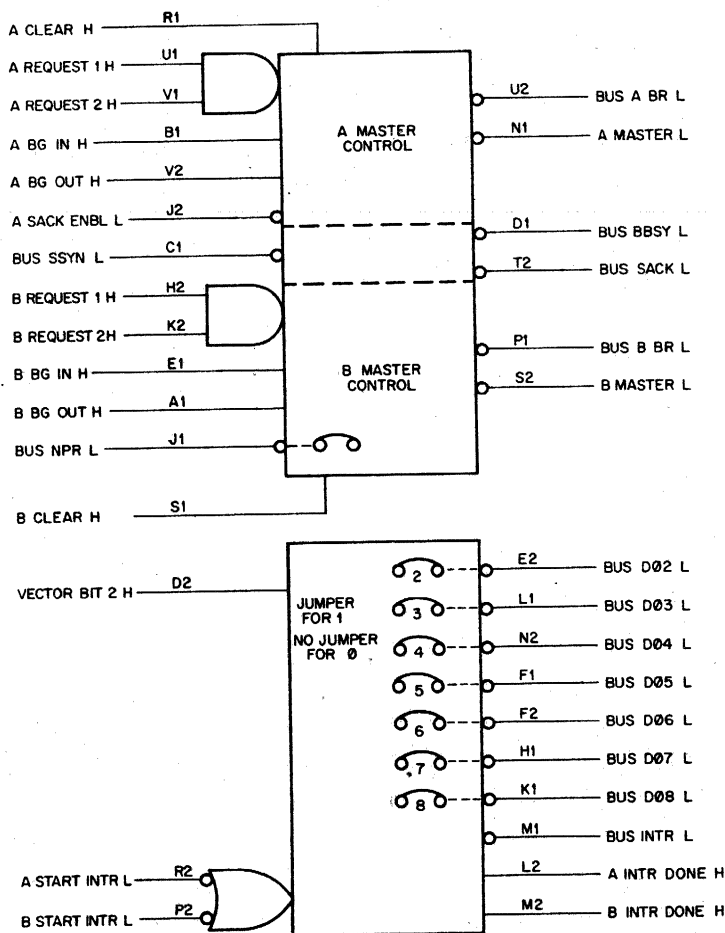
Figure 6-27 M7821 Interrupt Control Block Diagram
