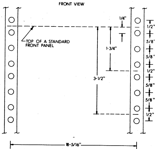
Standard PDP-11 Cabinet
