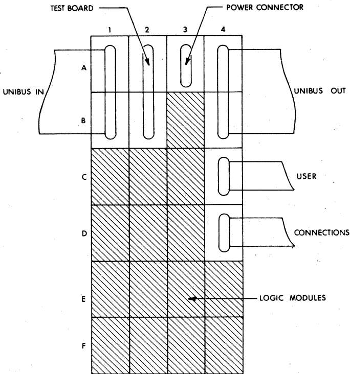
DR11-B System Unit
