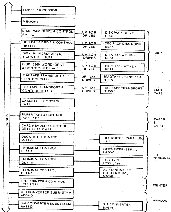
Figure 9-5 System Architecture of Major Components
