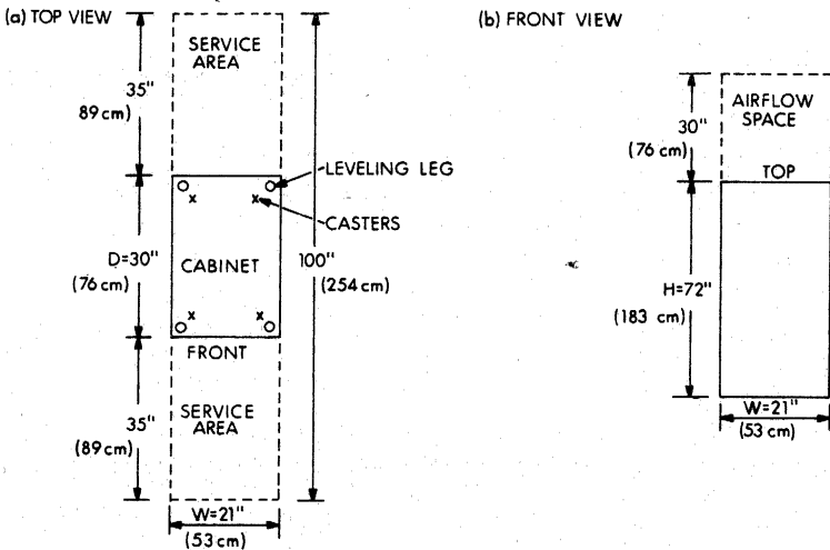
Figure 8-1 Space for 1 Cabinet
