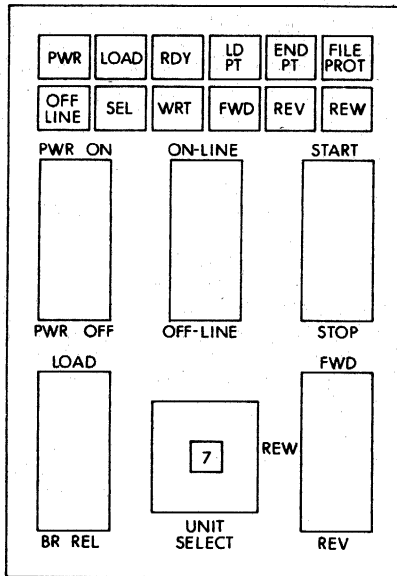
Operator Control Box
