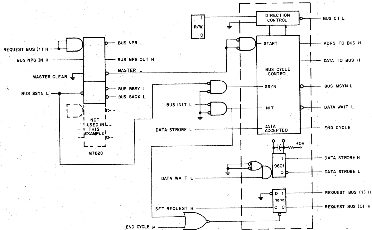
Figure 6-18 M796 UNIBUS Master Control (typical use) 6-21
