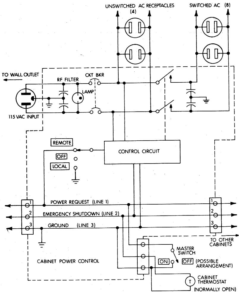
Figure 8-6 Power Control System
