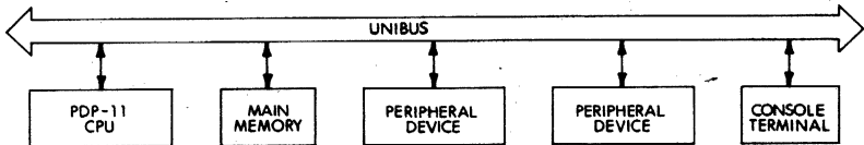
Figure 1-1 PDP-11 System Block Diagram
