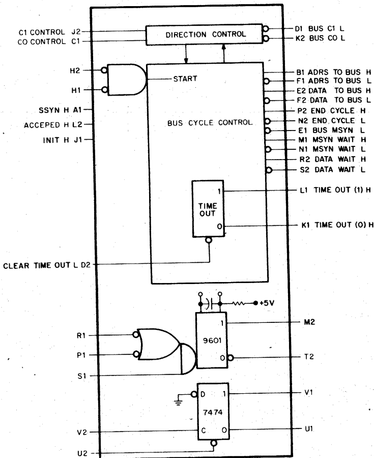
Figure 6-17 M796 UNIBUS Master Control (block diagram)
