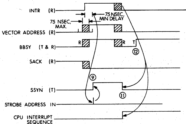
Figure 5-13 Interrupt Timing Diagram
