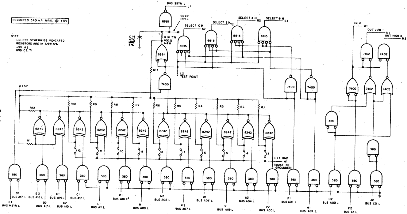
Figure 6-12 M105 Address Selector (schematic diagram)
