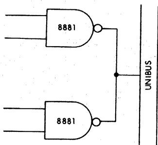
Figure 6-6 Wired OR Configuration
