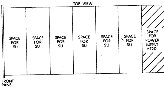
Figure 9-3 Extension Mounting Box (BA11)
