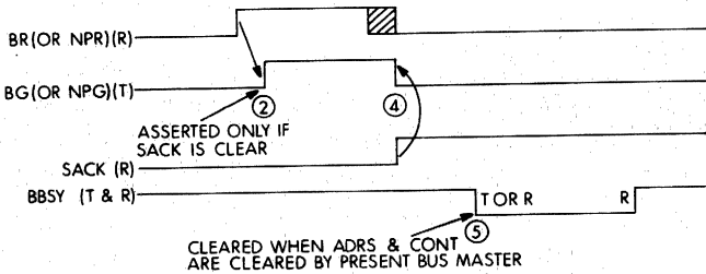
Figure 5-12 Priority Transfer Timing Diagram (nominally, for processor master)
