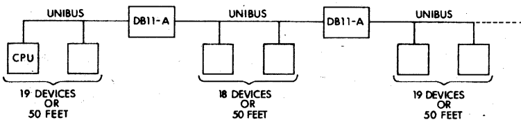
DB11 Bus Repeater
