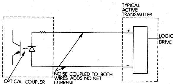
TTY RECEIVER WIRED AS PASSIVE
