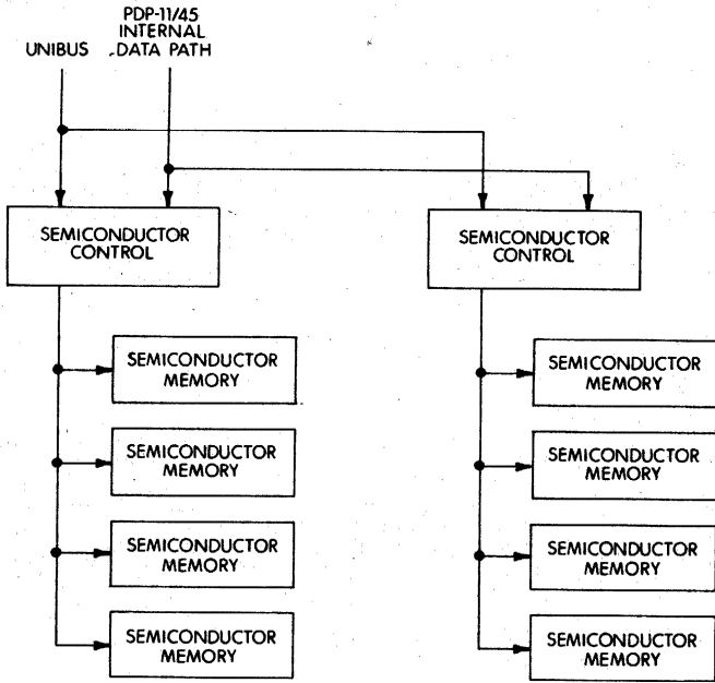
Block Diagram of Semiconductor Memory System
