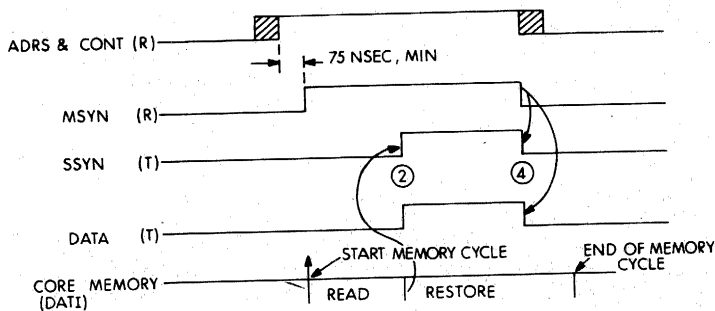
Figure 5-8 DATI & DATIP Timing Diagram
