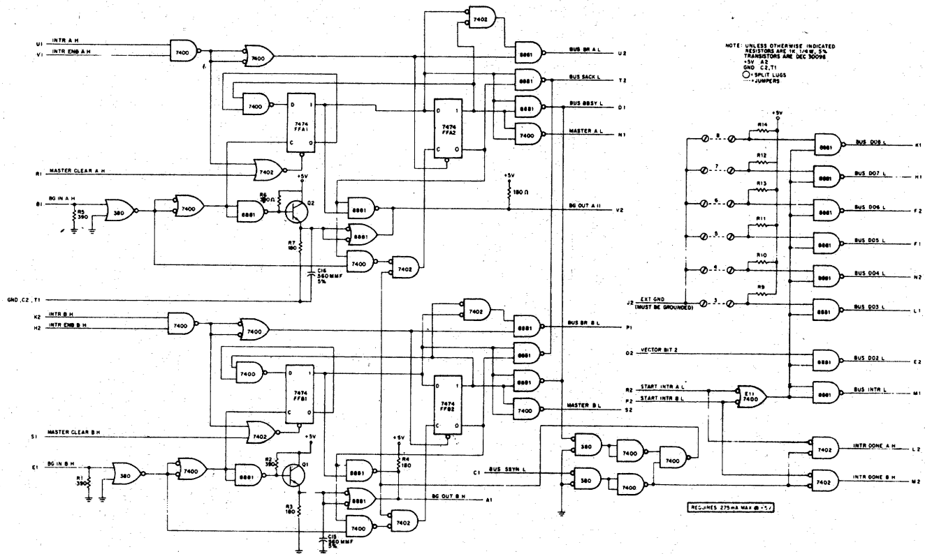
Figure 6-26 M7820 Interrupt Control (schematic diagram)
