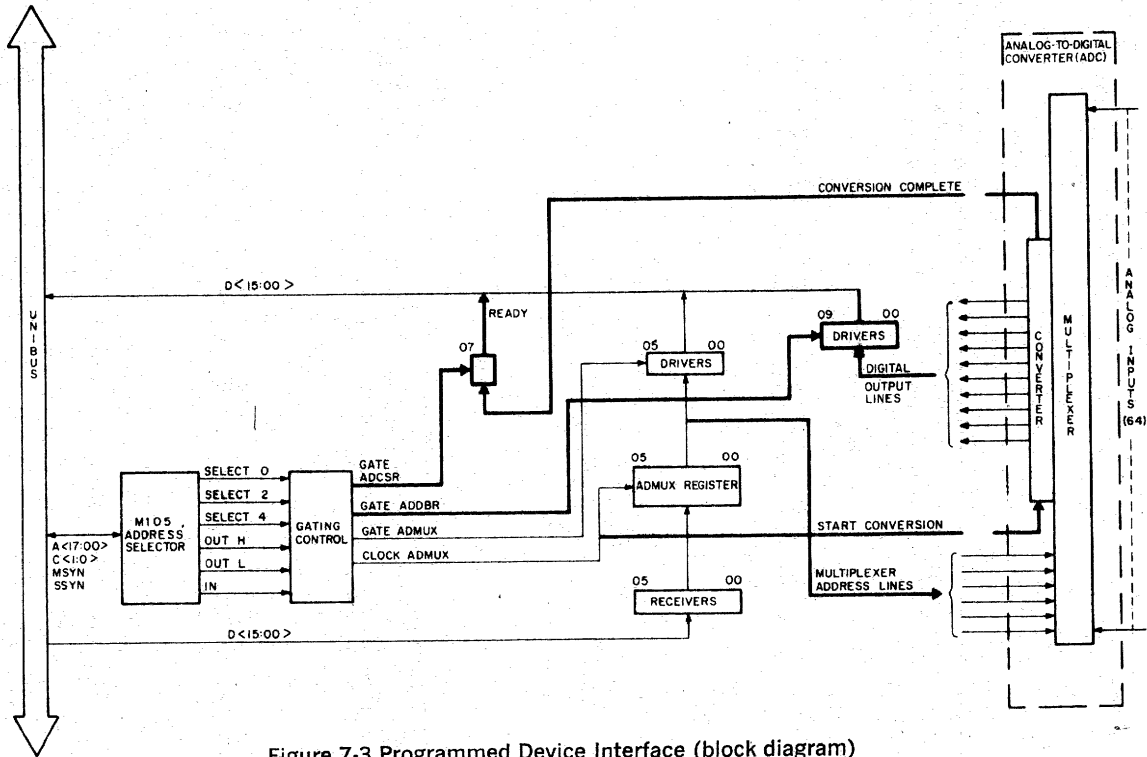
Figure 7-3 Programmed Device Interface (block diagram)
