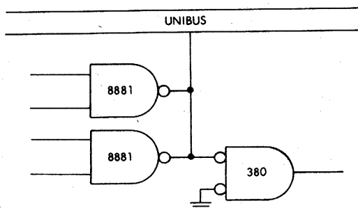
Figure 6-8 1 Bus Load
