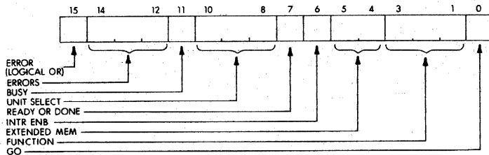
Figure 5-17 Preferred CSR Bit Assignments
