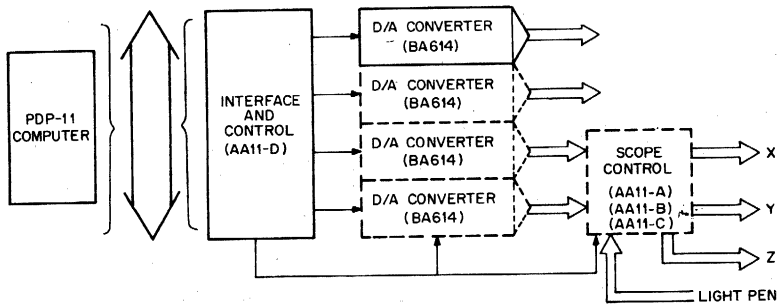
AA11-D Subsystem
