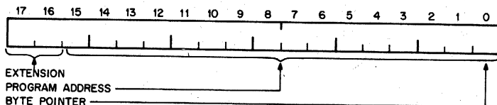
Figure 5-3 Address Line Bit Format
