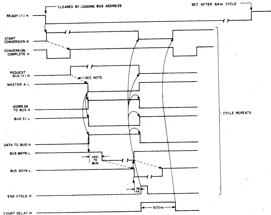
Figure 7-8 DMA Interface (timing diagram)
