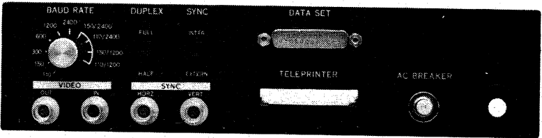
Rear Control Panel of the VT05
