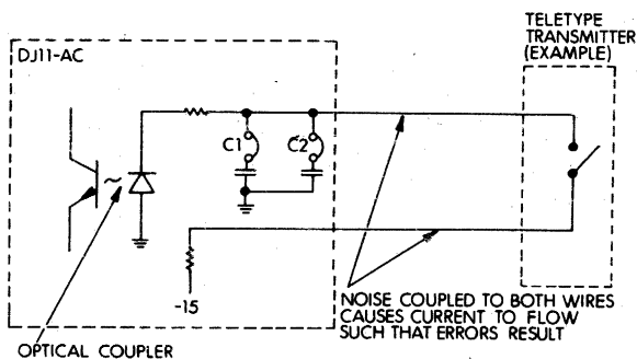
TTY RECEIVER WIRED AS ACTIVE
