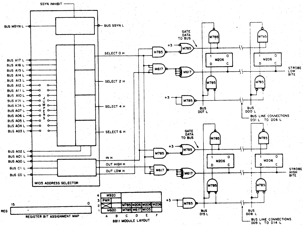
Figure 7-2 Basic Interface (schematic diagram)
