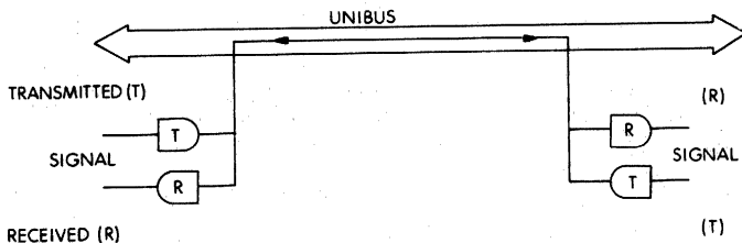
Figure 5-5 Bi-directional Signal
