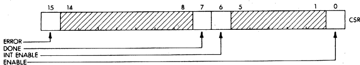
Figure 2-5 CSR Register
