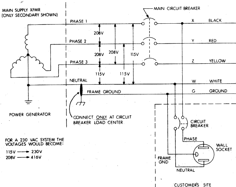
Figure 8-4 Power Wiring Schematic for 115 VAC
