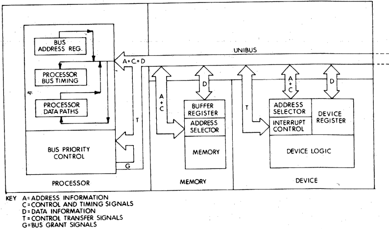
Figure 5-2 PDP-11 Interface Block Diagram
