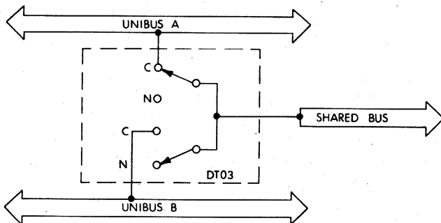
Equivalent Circuit of DT03
